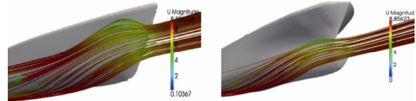
Fig. 13 Streamlines near the bows of hull 1 and hull 2
